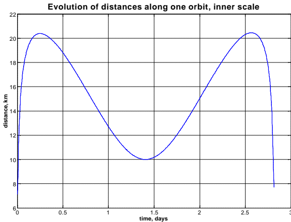
Figure 15: Evolution of Small-Scale S/C Distances over 1 Orbit
