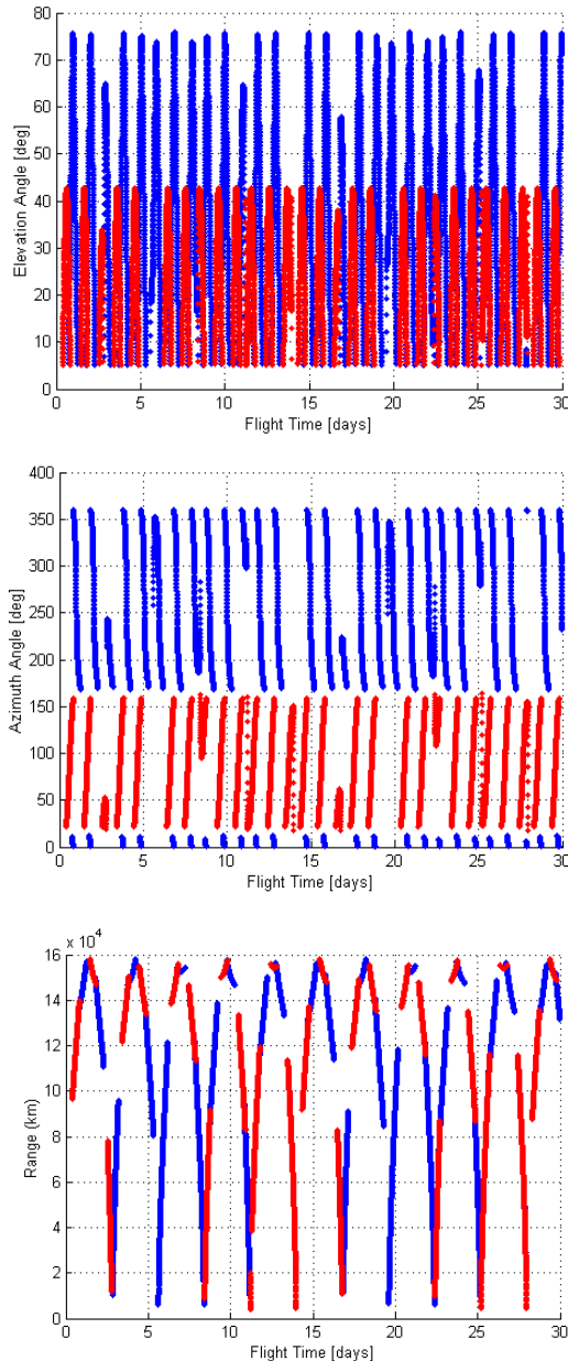
Figure 23: S/C Range, Elevation and Azimuth Angles during Maspalomas (blue) and Perth (red) Passes (min elevation = 5°)
